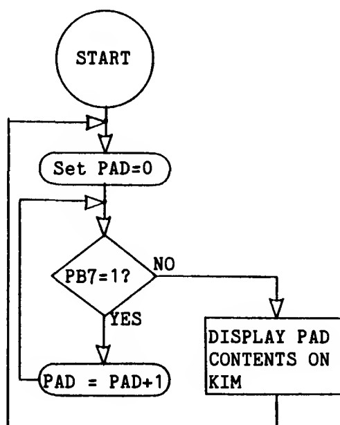
Flow Chart for Analog to Digital Converter
